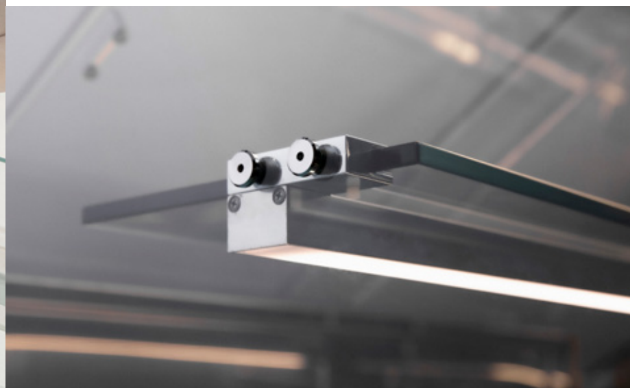
Fixed shelf clamp with integrated led light fixture
