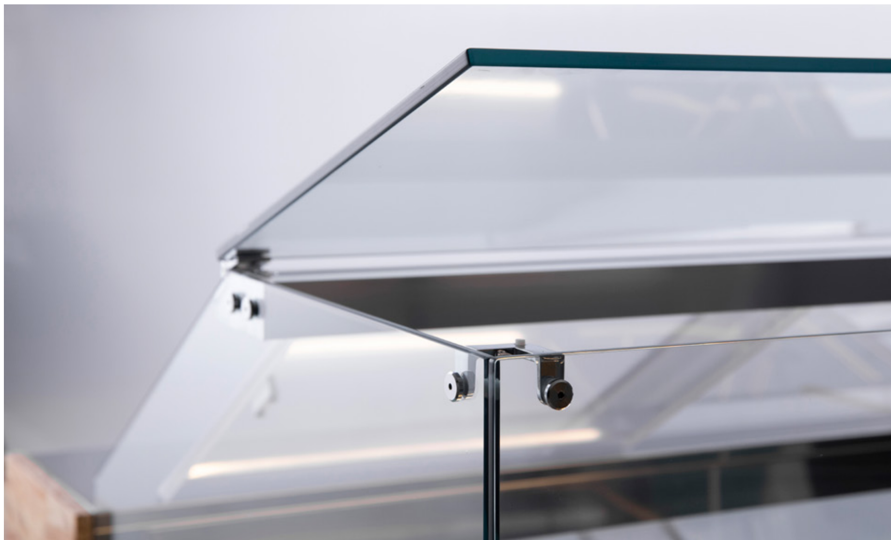
Micro-hinges and hardware for glass structure R4UP
